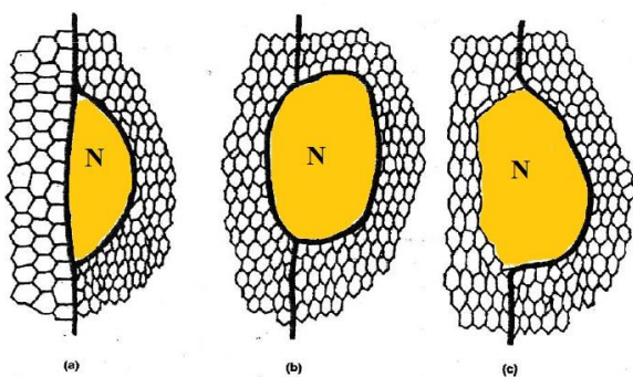
Fig. 39: Schematic showing three types of grain-boundary nucleation and the growth of the nucleus (N) at the expense of the polygonized subgrains. [17]
