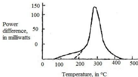
Fig. 1: (b) Anisothermal anneal curve. Electrolytic copper. (from Clarabrough, H. M., Hargreaves, M. E., and West, G. W., Proc. Roy. Soc. Lomdon , 232 A, 552 [1995]). [14]
