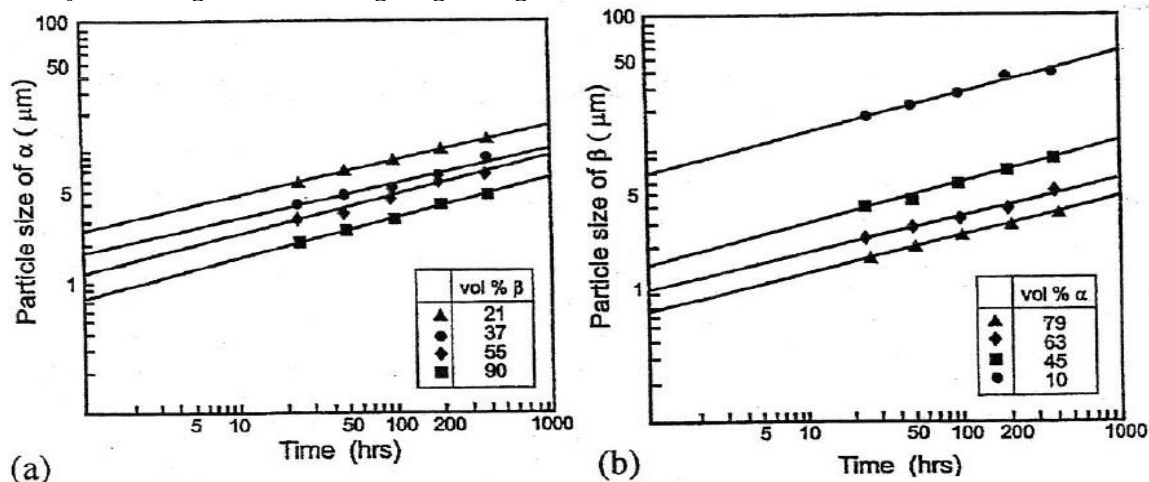
Fig. 41: (A) Growth kinetics of the phases in a series of Ti-Mn alloys containing different volume fractions at 973K, (a) \alpha phase, (b) \beta phase. (After Grewel and Ankem) {1989}. [19].
