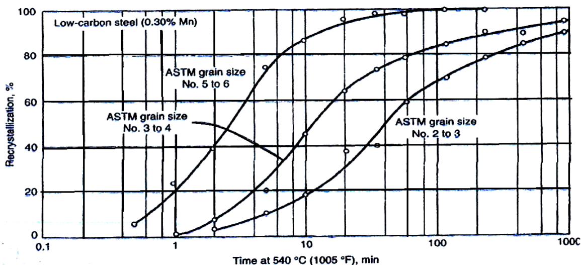
Fig. 38: Effect of penultimate grain size on the recrystallization kinetics of a low- carbon steel, cold rolled 60% and annealed at 540°C (1005°F). Note the incubation time is shortened as the penultimate grain size before cold rolling is decreased. [17]
