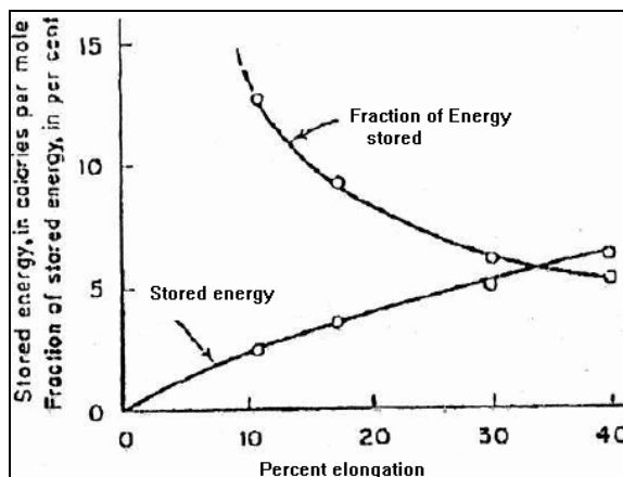
Fig. 1: (a) Stored energy of cold work and fraction of the total work of deformation remaining as stored energy for high purity copper plotted as functions of tensile elongation (From Data of Gordon, P., Trans.AIME, 203 1043 [1955]). [14].
