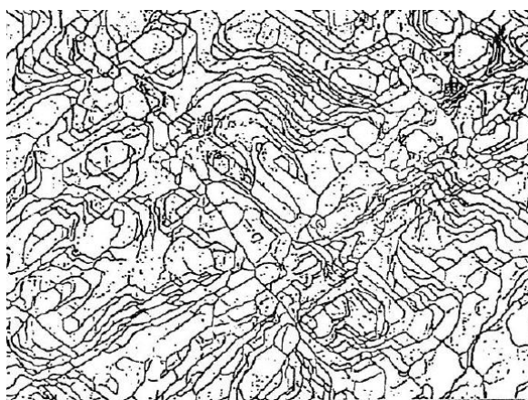
Fig. 14: Complex polygonized structure in a silicon-iron crystal that was deformed 8 percent by cold rolling before it was annealed 1hr at 1100°C. (Hibbard, W.R., Jr., and Dunn)
