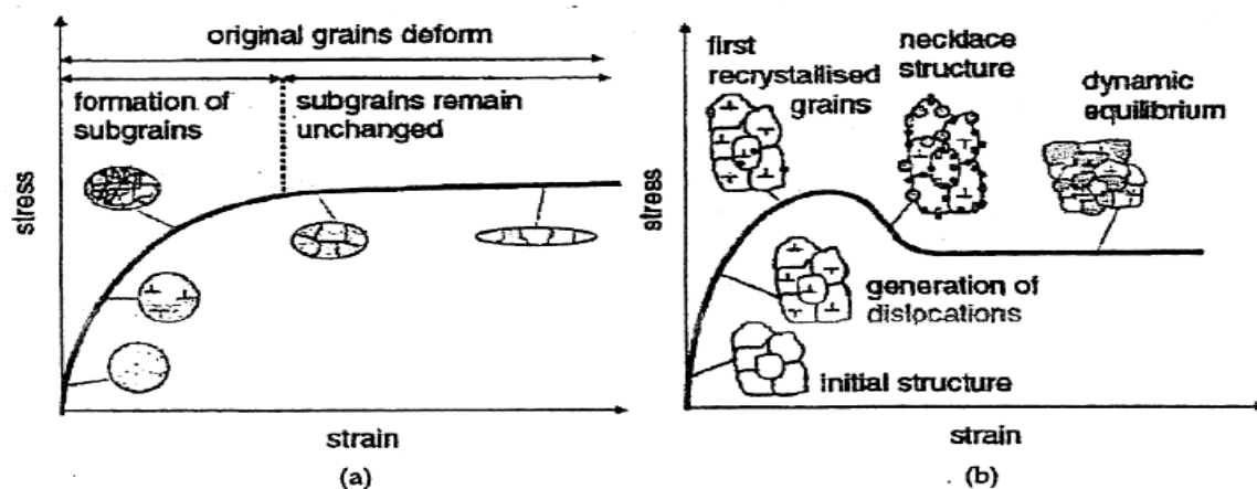
Fig. 36: Evaluation of the microstructure during (a) Hot deformation of a material showing recovery. (b) Continuous dynamic recrystallization (CDRX).
